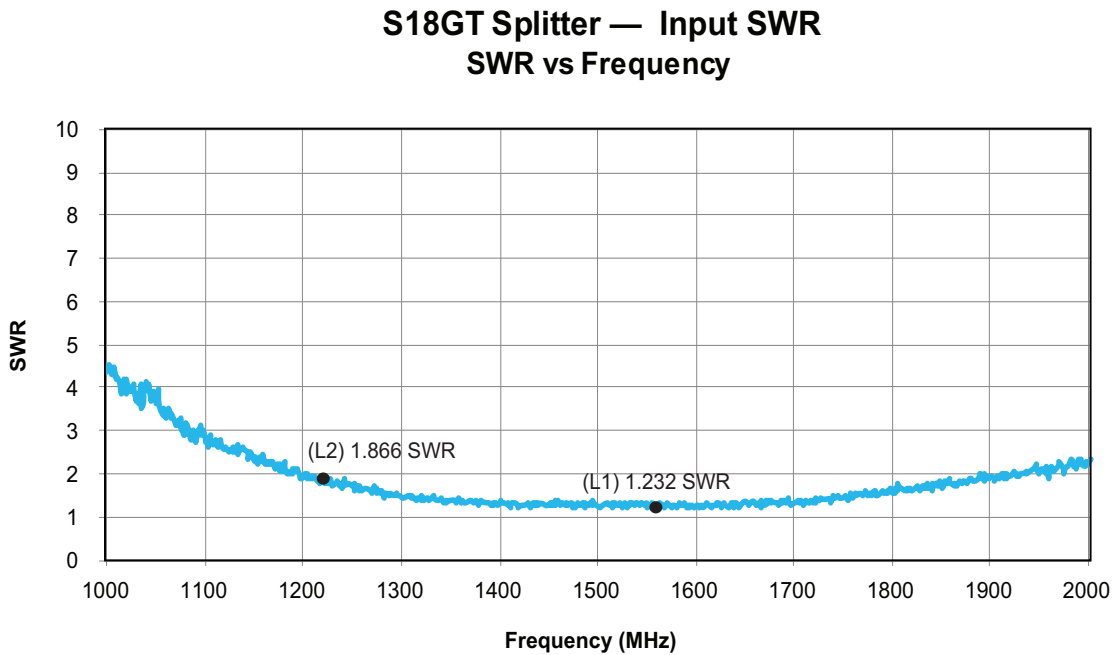
Figure 2-2. Input SWR
