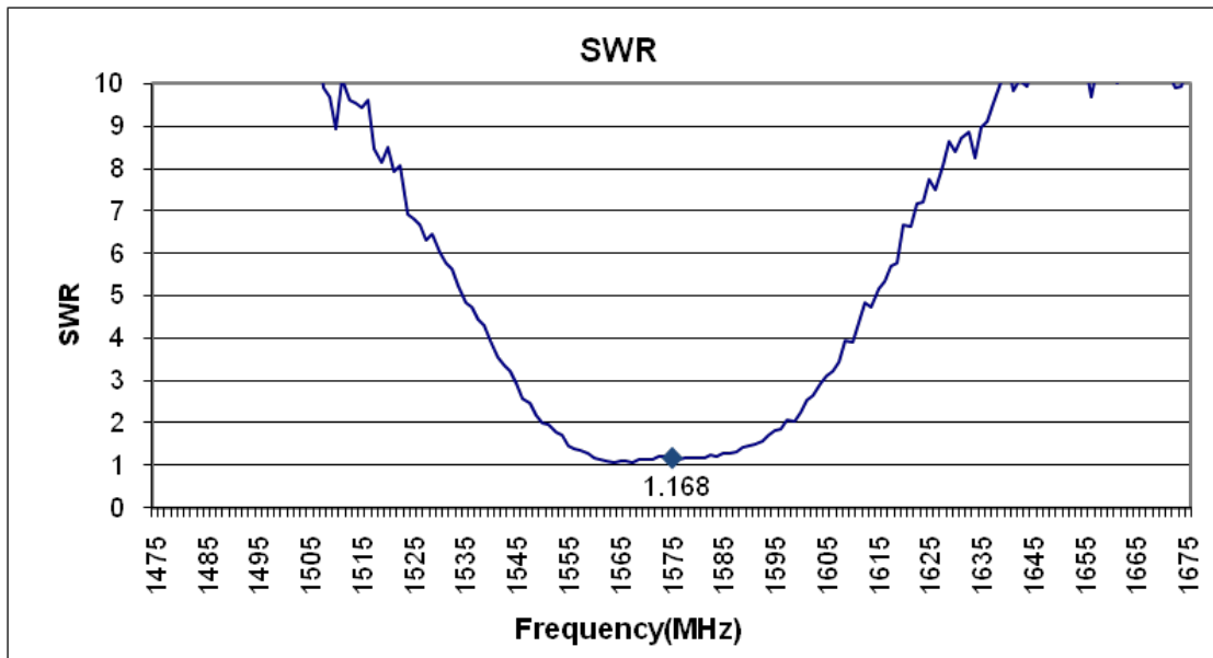
Figure 5. S14WI input SWR Performance (Filtered Option)
