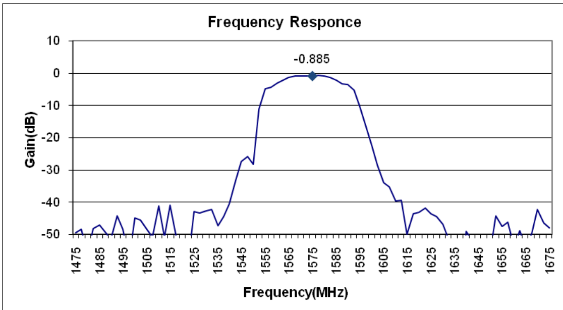
Figure 4. S14WI Output Port Performance (Filtered Option)
