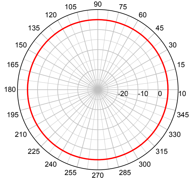
RMM at 1800 MHz – Azimuth Plot
