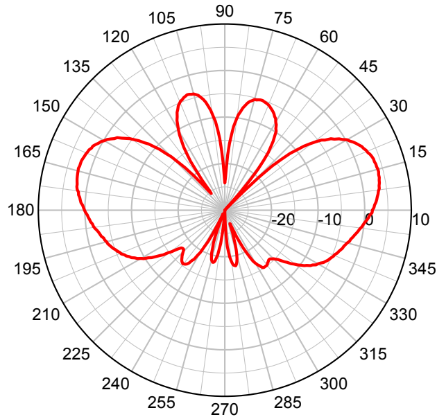
RMM at 2400 MHz – Elevation Plot
