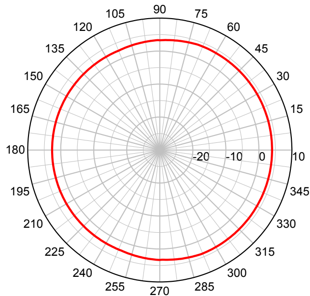
RMM at 2400 MHz – Azimuth Plot
