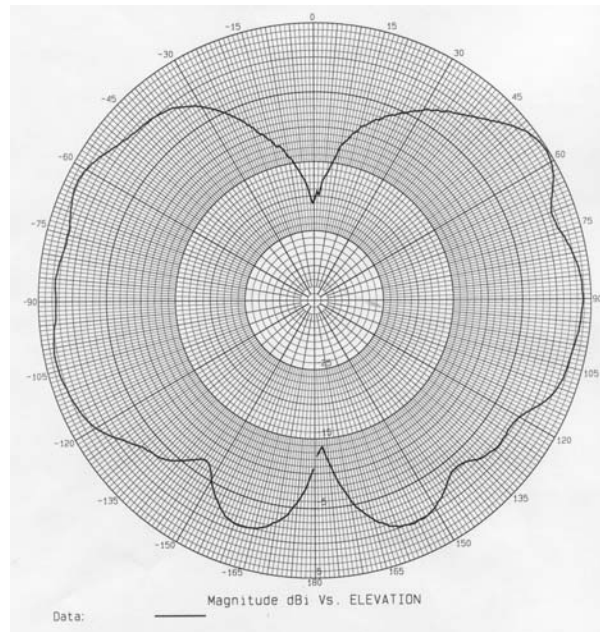
PSTN2 @ 5900 MHz– Elevation Plot
