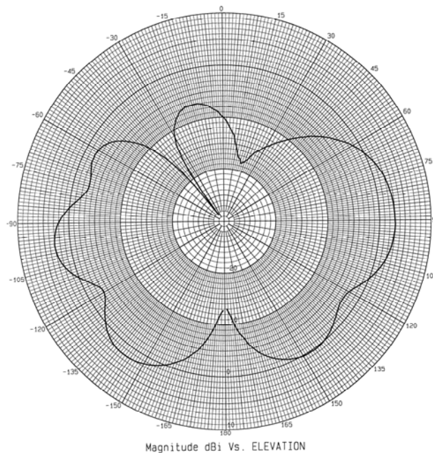
PSKN3-700/2100S- Typical Elevation Plot 1710-2170 MHz
