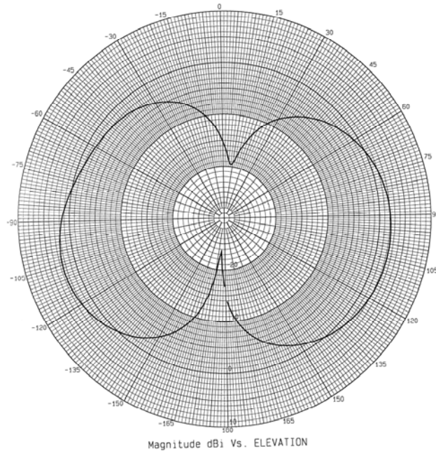
PSKN3-700/2100S- Typical Elevation Plot 694-960 MHz
