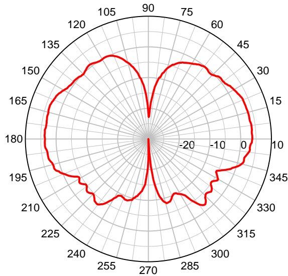
PSKN3-24/55 5-6 GHz Series – Elevation Plot
