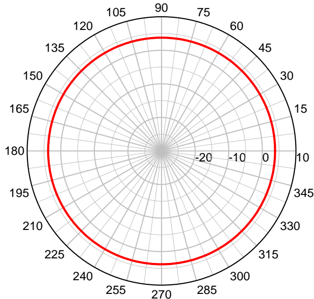
PSKN3-24/55 5-6 GHz Series – Azimuth Plot
