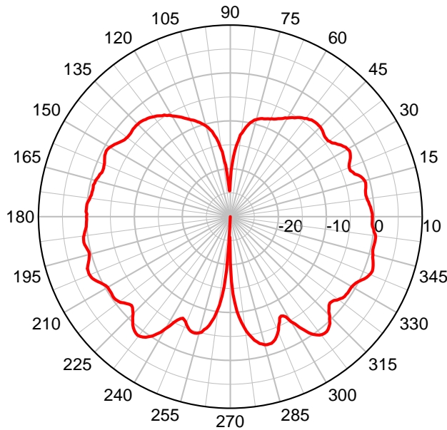
PSKN3-24/55 2.4 GHz Series – Elevation Plot
