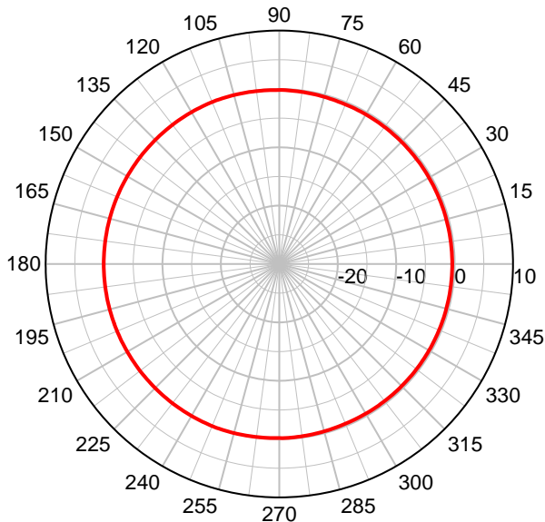
PSKN3-24/55 2.4 GHz Series – Azimuth Plot
