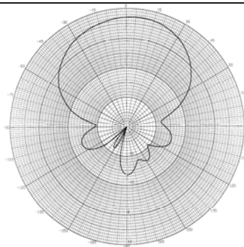
Azimuth Plot @ 2450 MHz
