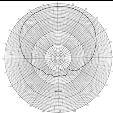
Azimuth Plot @ 2400 MHz
