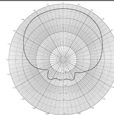
Azimuth Plot @ 2500 MHz
