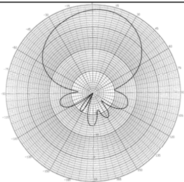
Azimuth Plot @ 2400 MHz
