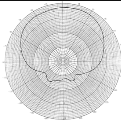
Azimuth Plot @ 2450 MHz
