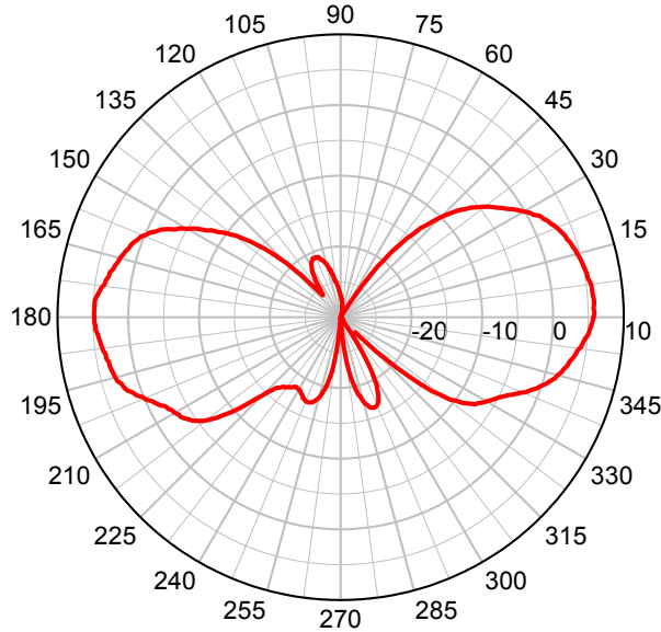
OD3-2400MOD2 – Elevation Plot
