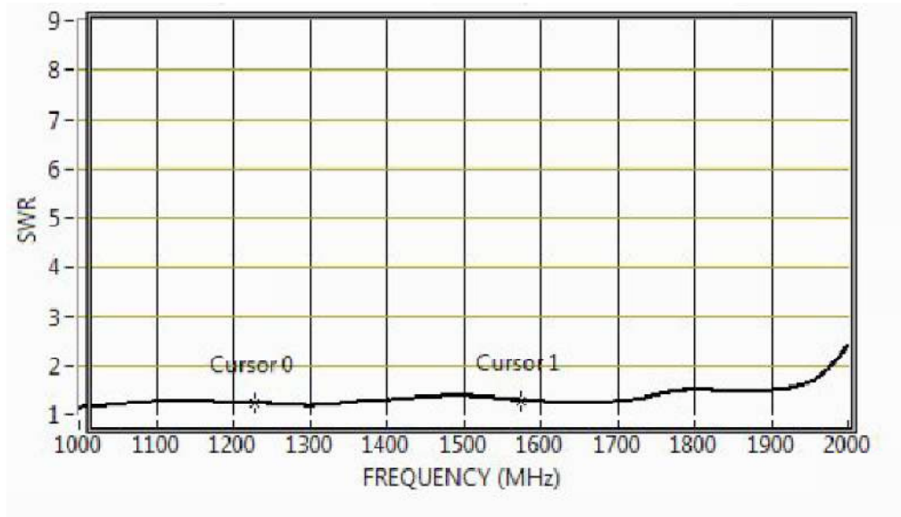
Figure 5. SWR vs. Frequency for Passive MS12 Splitter
