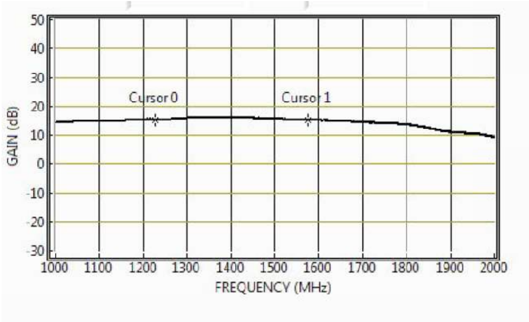
Figure 6. Gain vs. Frequency for Active MS12 Splitter
