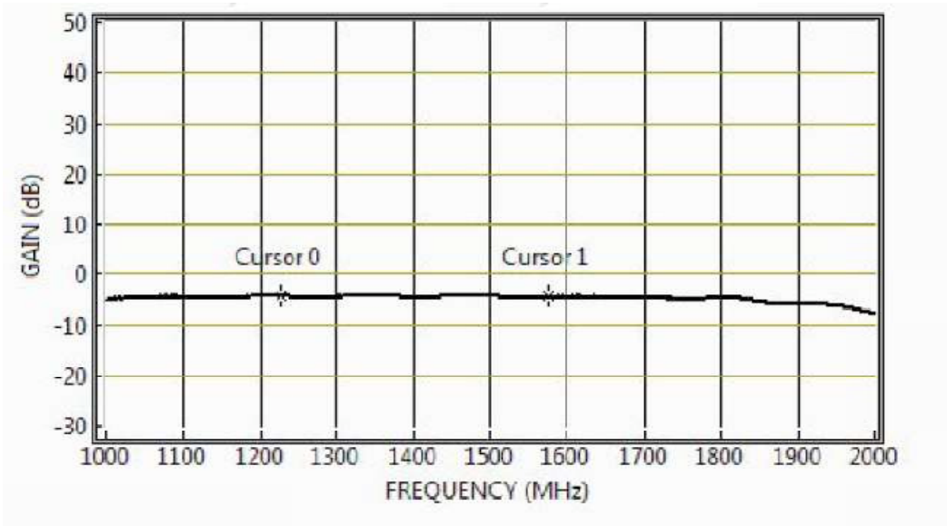
Figure 4. Gain vs. Frequency for Passive MS12 Splitter
