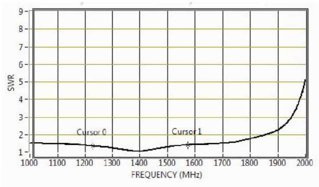
Figure 7. SWR vs. Frequency for Active MS12 Splitter
