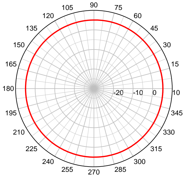
MRM3-5500 Series – Azimuth Plot
