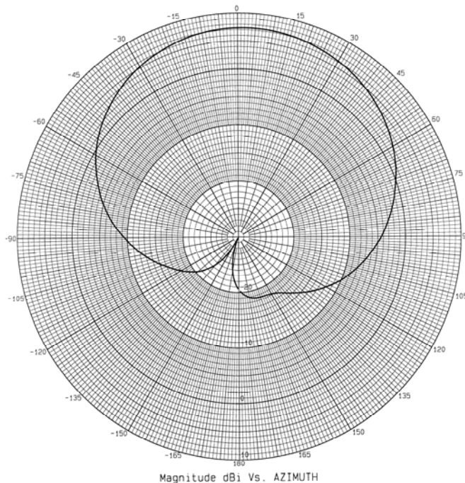
HD7-915RCP – Azimuth Plot
