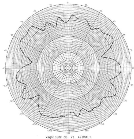
EM@5500 MHz – Azimuth Plot
