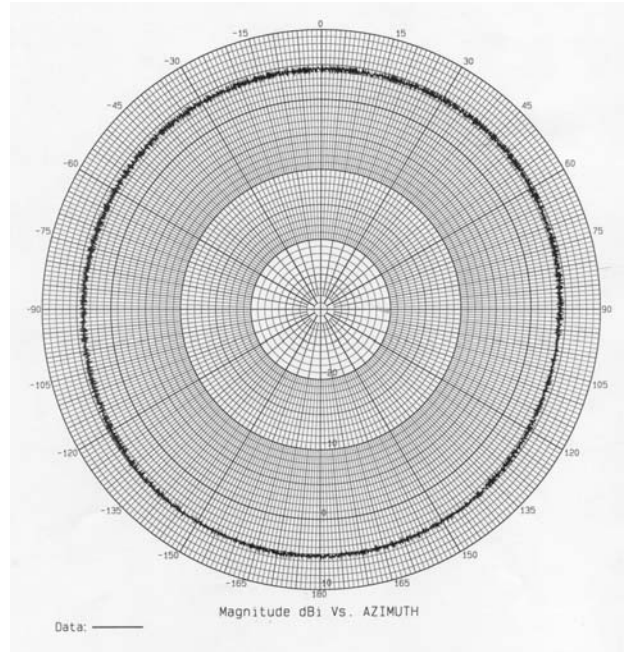
ECO5-2400/5500 – Azimuth Plot @ 5500 MHz
