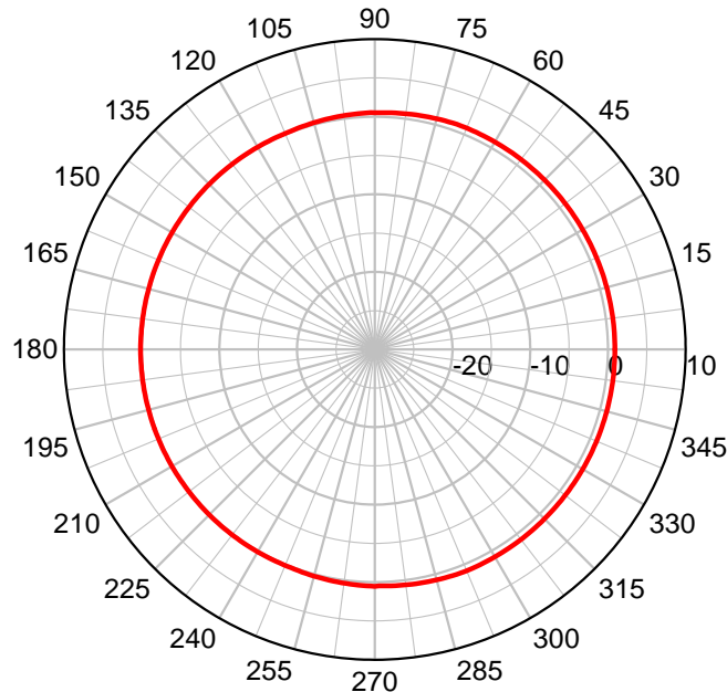
CVS 915 Series – Azimuth Plot
