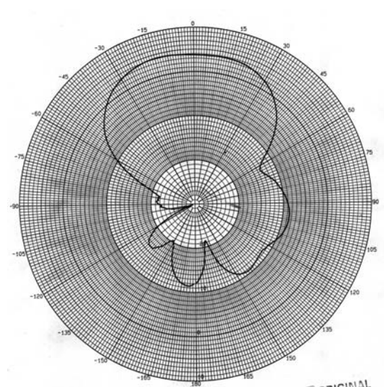
CVO @ 1900 MHz – Elevation Plot
