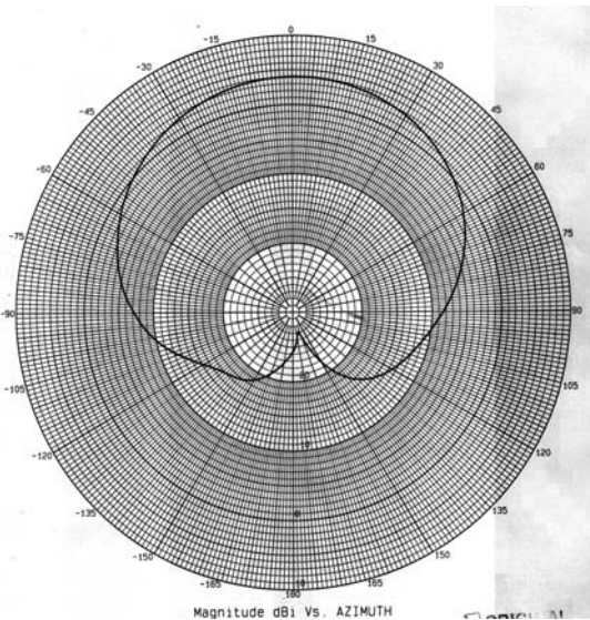
CVO @ 850 MHz – Azimuth Plot
