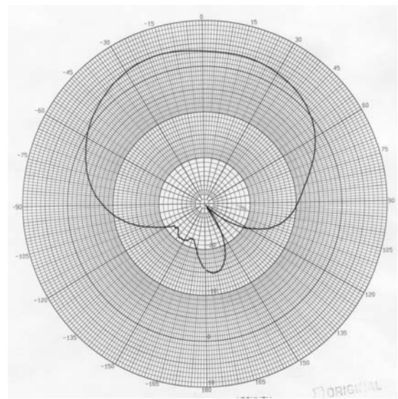
CVO @ 1900 MHz – Azimuth Plot
