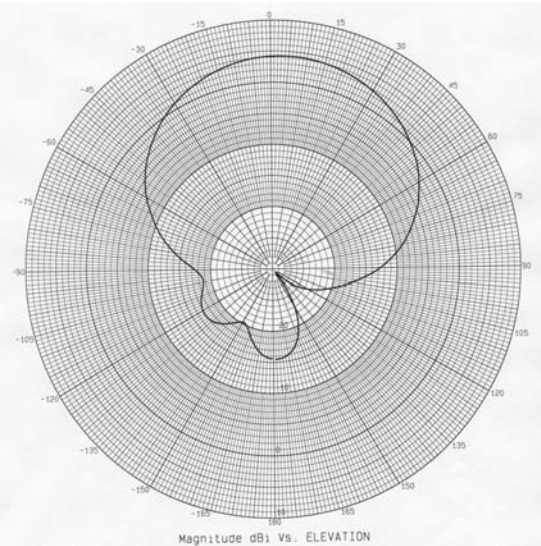
CVO @ 850 MHz – Elevation Plot
